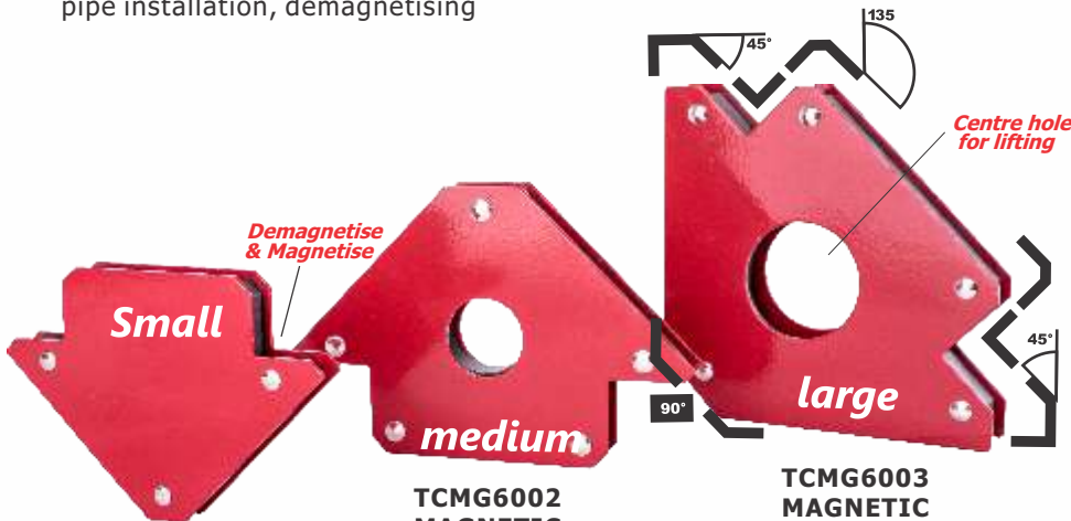
TCMG6001 MAGNETIC Welding Holder 11.4kg Pull Force 45, 90 & 135° Multi Angle
